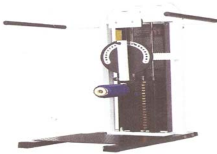
KL 622 Multi-hip Machine 120 x 118 x 157 cm
